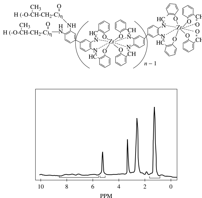
Figure 3.31 The copolymerization reaction between \text{Zr}(\text{tsdb})_n and (\pm)\beta -butyrolactone and the proton NMR spectrum of the product. (Spectrum taken by B. Wang.)
