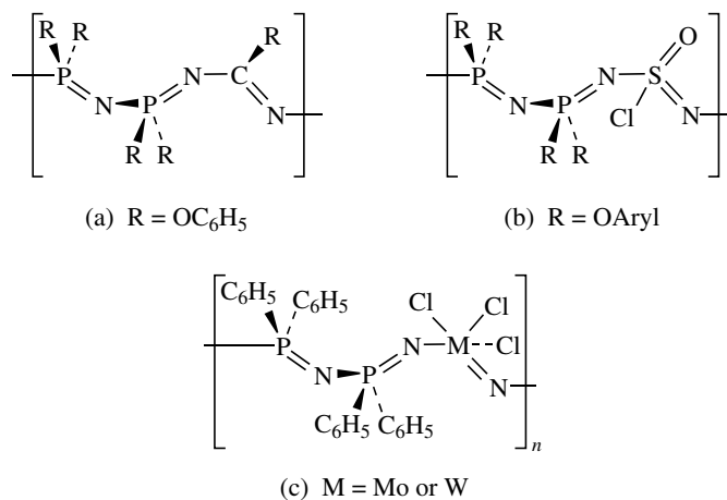
Figure 1.27 Polyheterophosphazenes: (a) a polycarbophosphazene; (b) a polythiophosphazene; and (c) a metallophosphazene.
