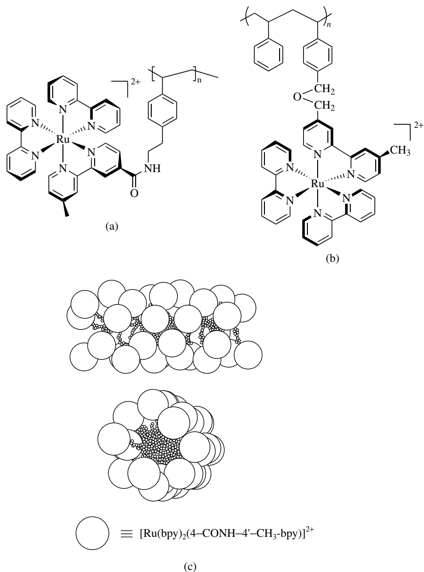
Figure 4.19 Anchored ruthenium(II) polymers: (a) amide linkage to bis(2,2'-bipyridine) (4-carbonyl-4'-methyl-2,2'-bipyridine)ruthenium(II) (reprinted with permission from Ref. 106; © 1998 American Chemical Society); (b) similar species with ether linkage (reprinted with permission from Ref. 105; © 1999 American Chemical Society); and (c) energy-minimized end-on and side views of polystyrene amide linked to a ruthenium polymeric cation, probably a [(\text{PS-4-derivatized-4'-methyl-2,2'-bipyridine})(2,2'\text{-bipyridine})_2\text{Ru}^{\text{II}}]_{30}^{60+} type ion, based on modified MM2 parameters and CAChe software (reprinted with permission from Ref. 106; © 1998 American Chemical Society). [(c) is not the \text{Ru}^{\text{II}}]_{18}^{36+} type ion claimed in the paper—more than 18 Ru centers are shown.]
