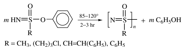
Figure 2.20 The synthesis of poly(alkyl/aryloxothiazenes).
