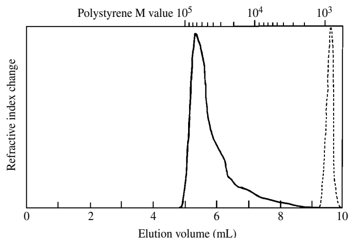
Figure 3.7 Gel permeation chromatogram of a metal coordination polymer prepared by step polymerization—poly(1,2,4,5-tetraaminobenzenezirconium(IV)) in NMP with a 10^3 Å Ultrastaygel® column. (chromatogram by C. J. Hardiman).
