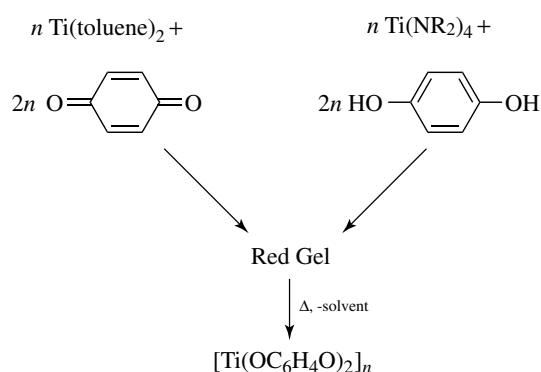
Figure 2.45 Oxidative addition and condensation polymerization pathways for the synthesis of [\text{Ti}(\text{OC}_6\text{H}_4\text{O})_2]_n (86).
