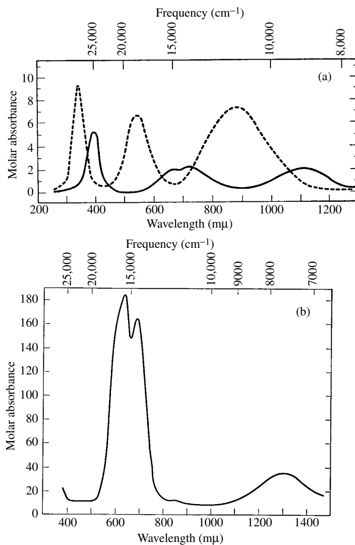
Figure 3.37 Typical visible and near-infrared absorption spectra for nickel(II) ions surrounded by ligands with different geometrical arrangements: (a) octahedral aqua [Ni(H 2 O) 6 ] 2+ (—) and ethylenediamine [Ni(NH 2 CH 2 CH 2 NH 2 ) 3 ] 2+ (---) ions; (b) tetrahedral Ni(Ph 3 AsO) 2 Br 2 , where Ph = C 6 H 5 . Spectra based on F. A. Cotton and G. Wilkinson, Advanced Inorganic Chemistry , 1st Ed., Wiley, NY, 1962, pp 735–736.
