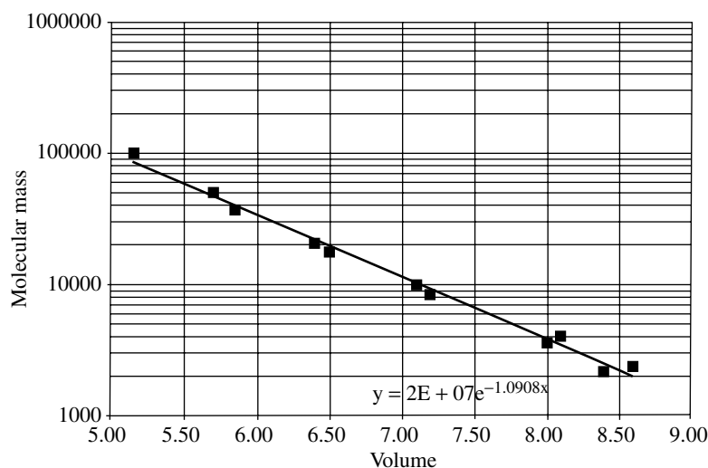
Figure 3.6 Example of a gel permeation chromatography column calibration curve — a 10^3 Å Ultrastyrigel® column using monodisperse polystyrene standards in NMP. (Calibration by C. J. Hardiman).
