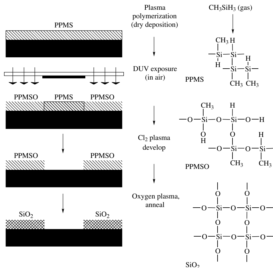
Figure 4.14 The process sequence for plasma polymerized methyl silane resists. A metallic conductor would be added between the SiO 2 insulators (58).
