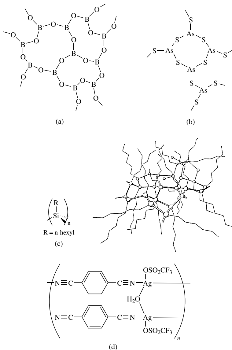
Figure 1.5 Examples of connectivity of 3: (a) boric acid, (b) arsenic(III) sulfide, (c) a synthetic polysilyne (Reprinted with permission from Bianconi et al., Macromolecules , 1989, 22 , 1697; © 1989 American Chemical Society); and (d) a synthetic silver polymer (Venkataraman et al., Acta Cryst. 1996, C52 , 2416).
