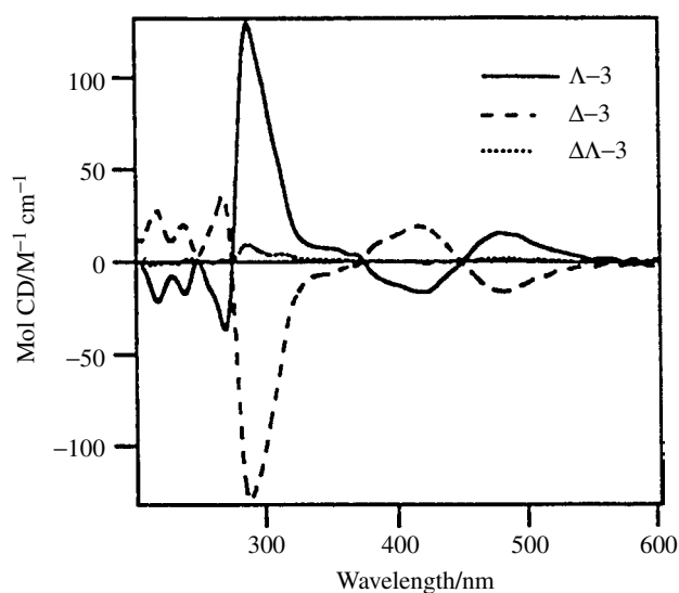
Figure 3.52 The circular dichroism (CD) spectra of \Lambda -, \Delta -, and \Delta , \Lambda ( meso )-catenapoly(2,2'-bipyridineruthenium(II)- \mu -tetrapyrrodo[3,2-a:2',3'-c:3''2''-h:2''',3''']phenazine hexafluorophosphate in acetonitrile. From Chen and MacDonnell, Chem. Commun. 1999, 2529; reproduced by permission of The Royal Society of Chemistry.
