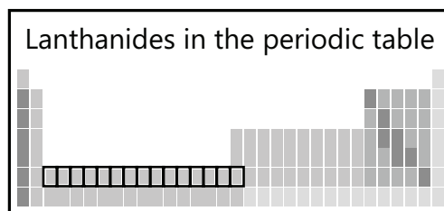
Figure 31.4: Position of lanthanides in the periodic table
