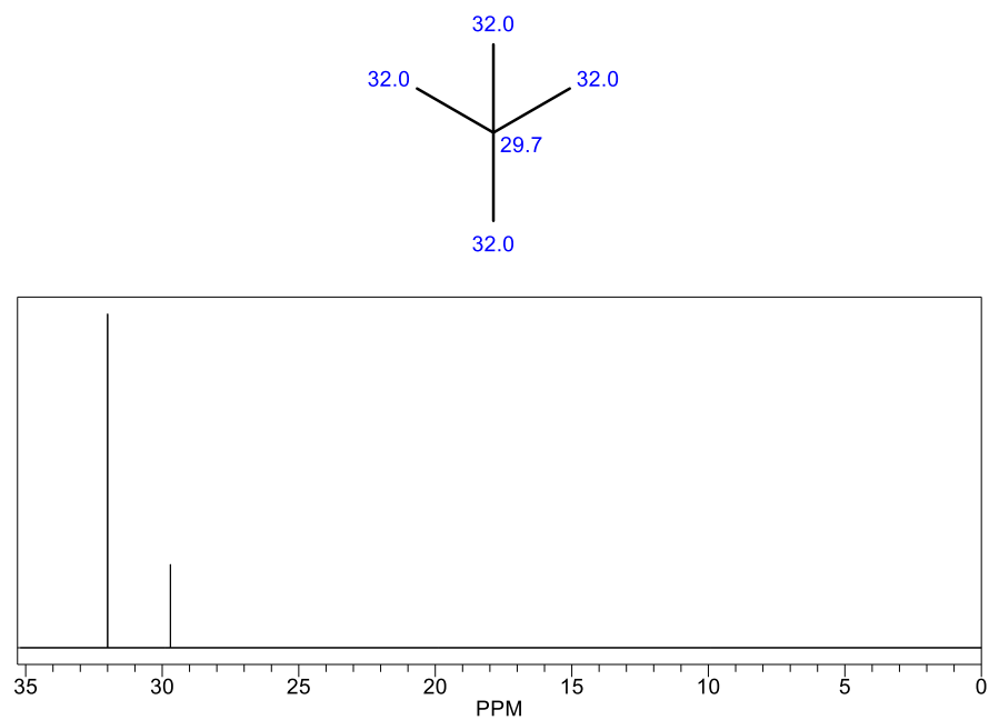
Proton Decoupled 13 C of Neopentane
