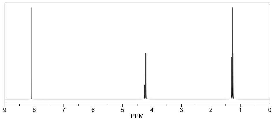
^1\text{H} Spectra of Ethylformate
