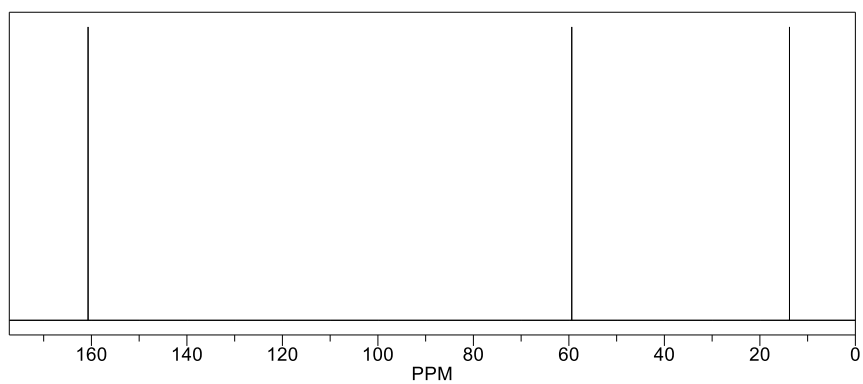
Proton Decoupled ^{13}\text{C} of Ethylformate
