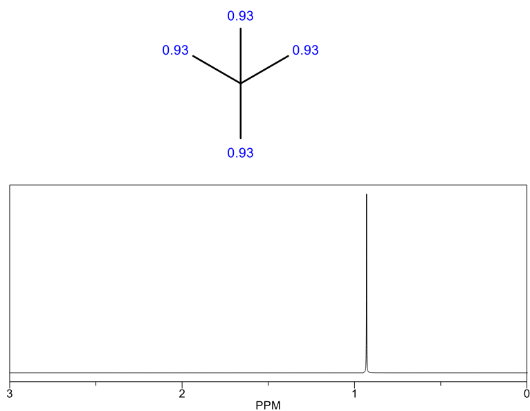
1 H Spectra of Isopentane
