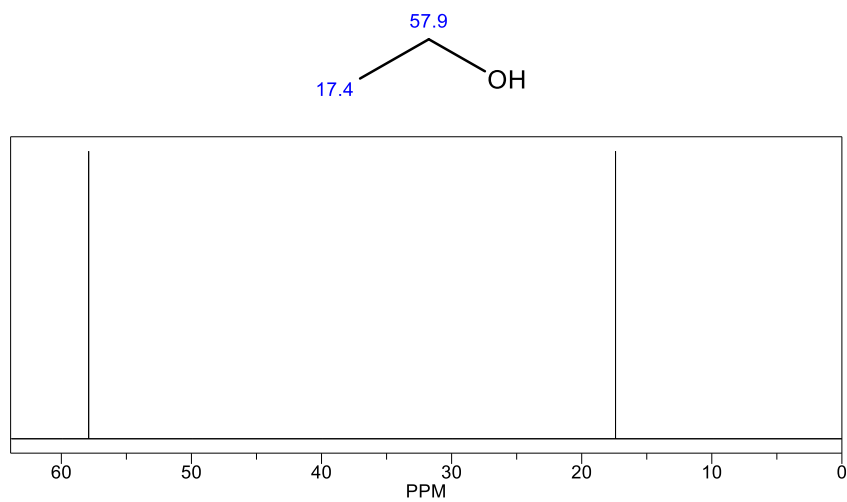
Proton Decoupled ^{13}\text{C} of Ethanol
