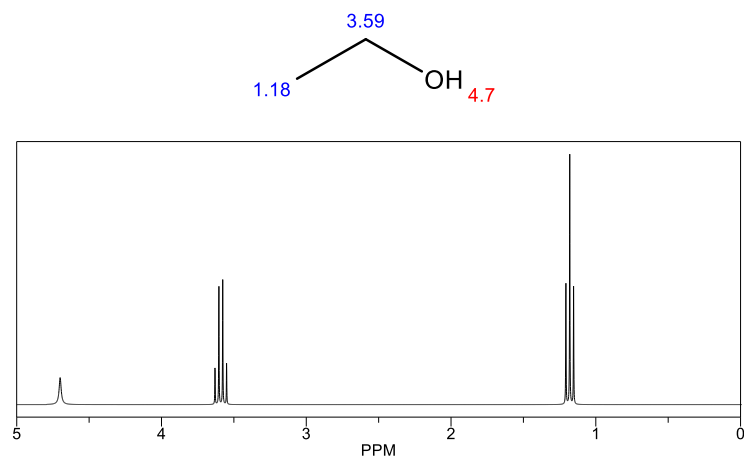
^1\text{H} of Ethanol
