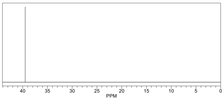
Proton Decoupled 13 C of Oxirane
