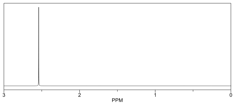
1 H Spectra of Oxirane
