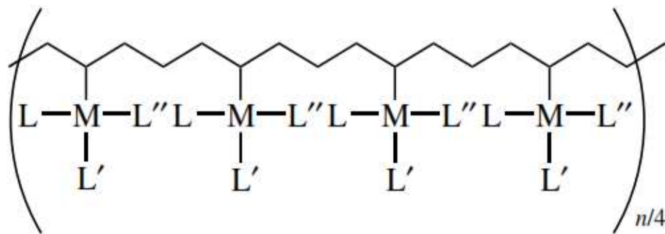
Figure 1.1 Schematic of anchored metal-containing polymer with a connectivity of 1, where M might be palladium or platinum with three other ligands. For catalytic activity, at least one of the three must be easily removed by a substrate.
