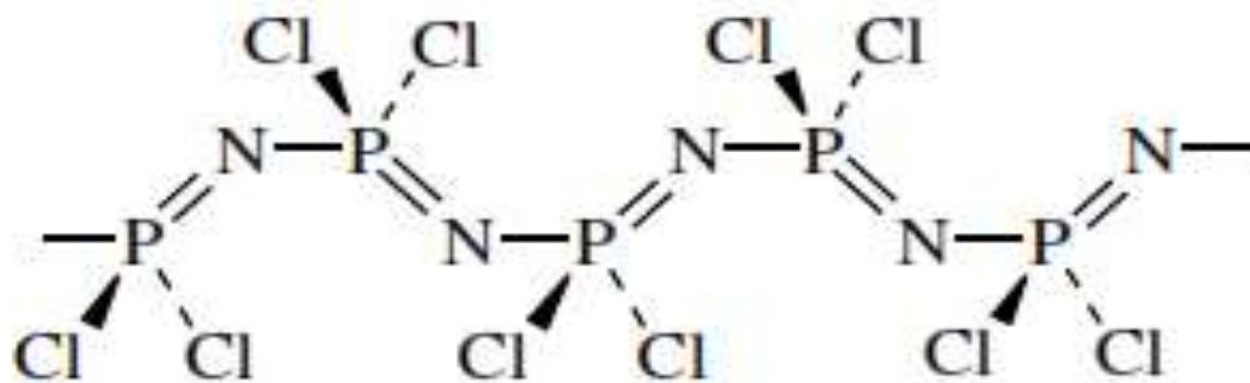
(c) poly(dichlorophosphazene)
